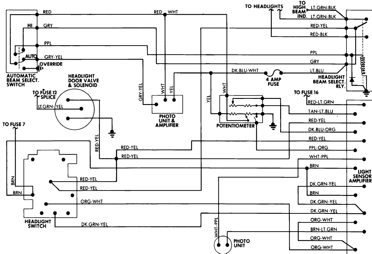
Lincoln Continental Automatic Headlights Autolamp Wiring Diagram
