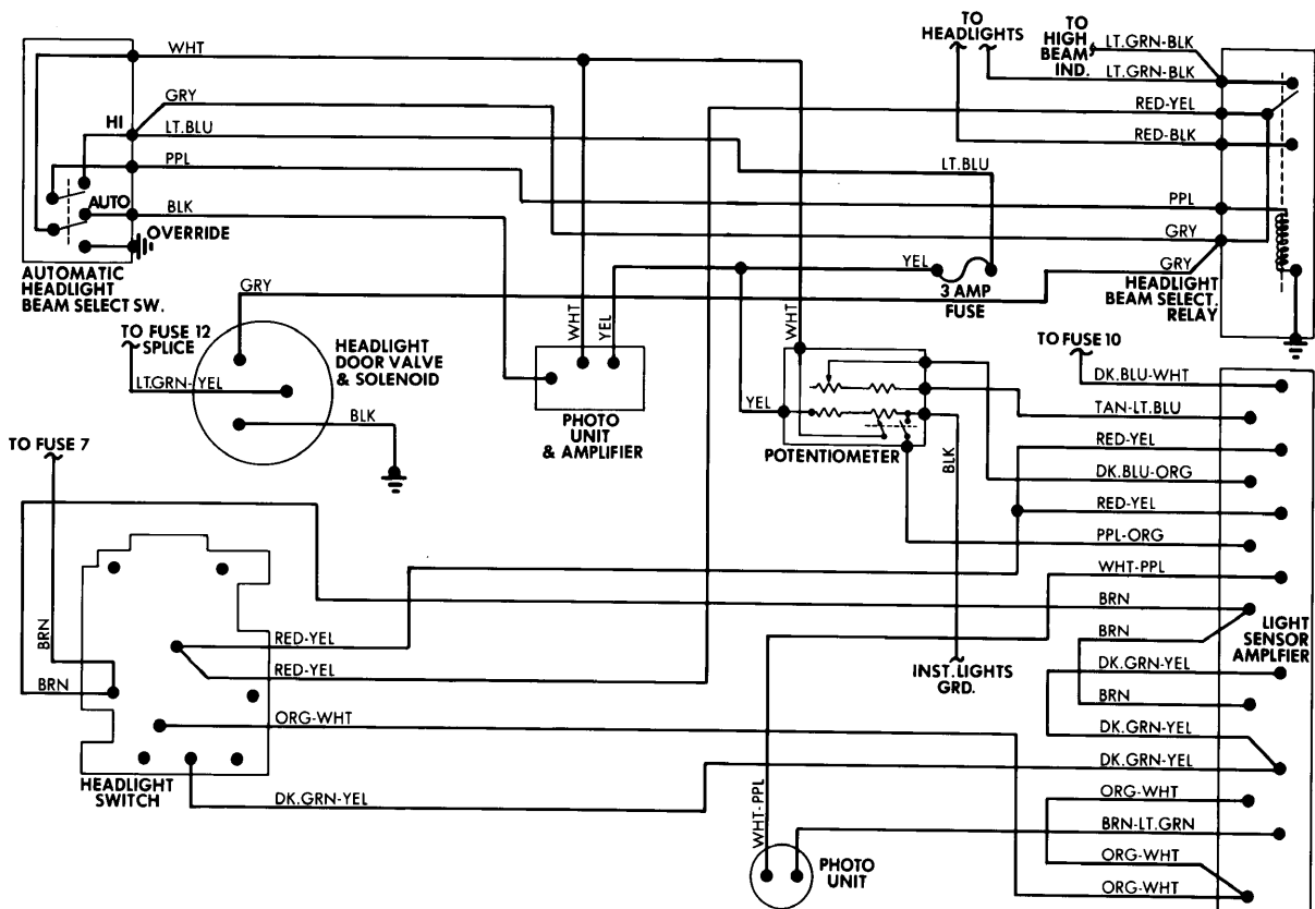
Lincoln Continental Mark V Automatic Headlights Autolamp Wiring Diagram
