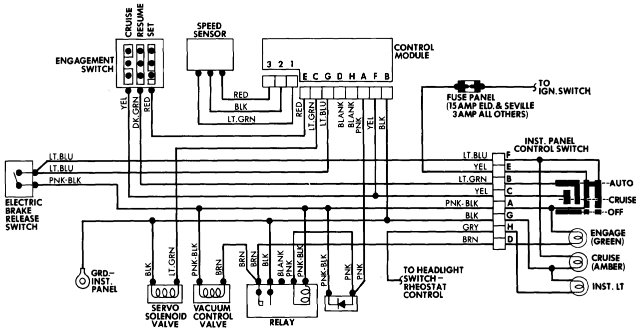
General Motors (Cadillac) Electronic Cruise Control Automatic Speed Control System Wiring Diagram
