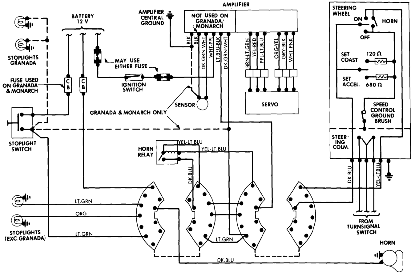
Ford Motor Co. Automatic Speed Control System Wiring Diagram
