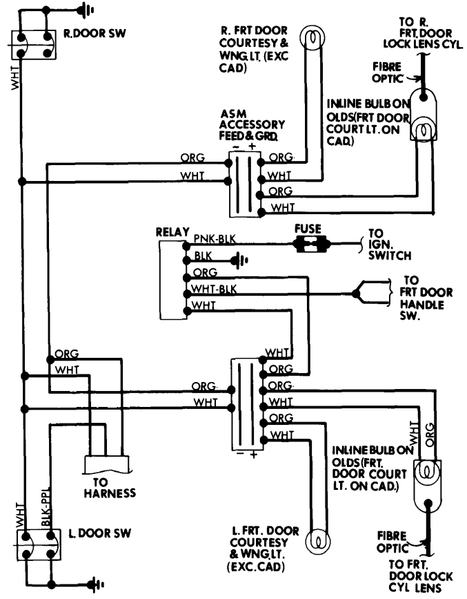
General Motors Lighted Door Lock and Lighted Entry System Wiring Diagram
