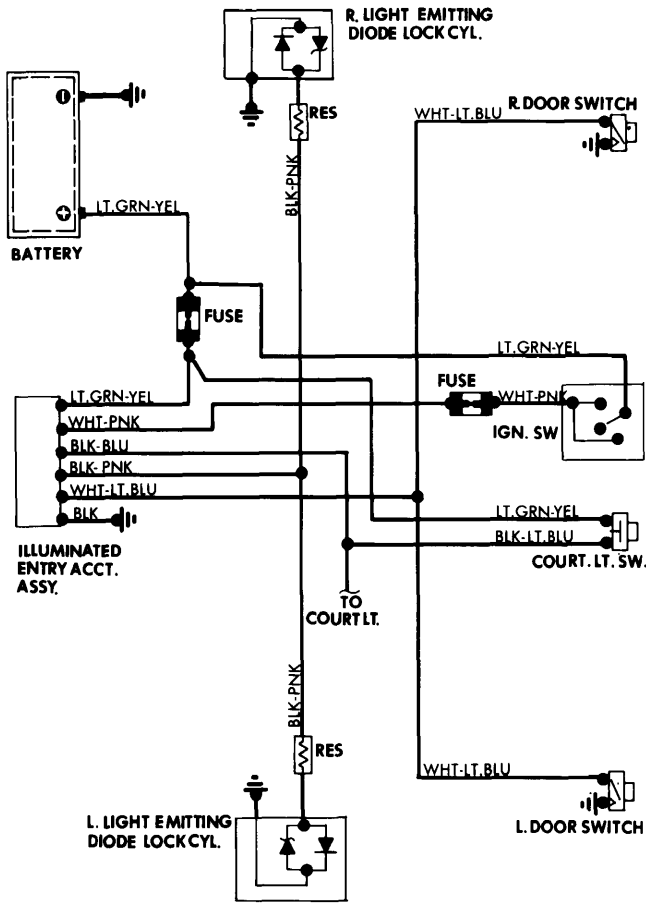
Ford Motor Co. Lighted Door Lock and Lighted Entry System Wiring Diagram
