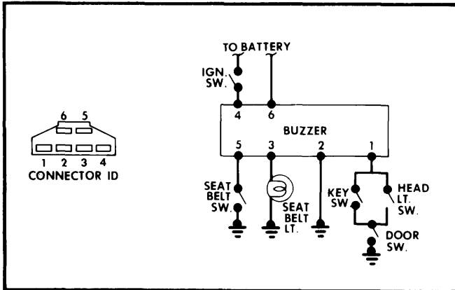
Key and Seat Belt Warning System Wiring Diagram for Chrysler Corp.
