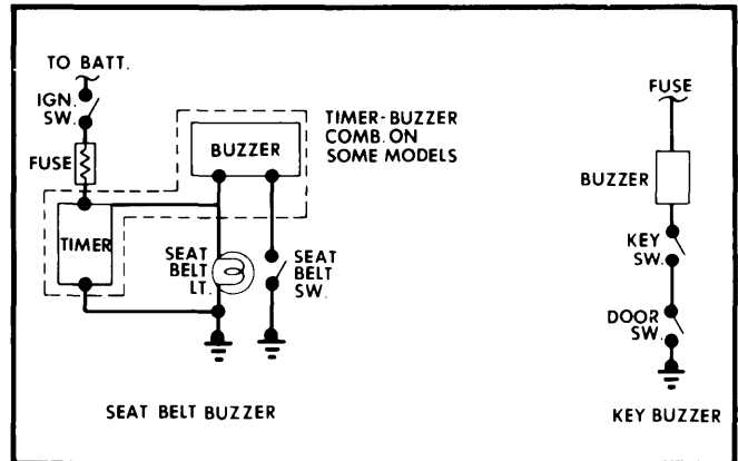
Key and Seat Belt Warning System Wiring Diagram for General Motors
