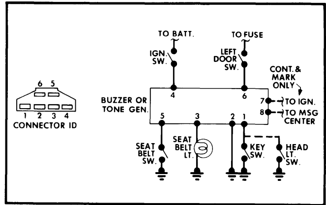
Key and Seat Belt Warning System Wiring Diagram for Ford Motor Co.
