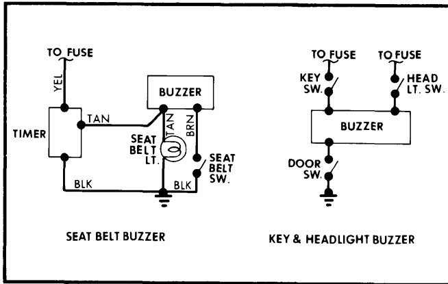
Key and Seat Belt Warning System Wiring Diagram for American Motors
